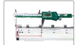
check lower jaws of caliper
