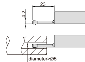
small hole probe (optional), code ISR-C002-PROBE
