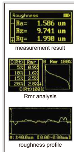
screen display
