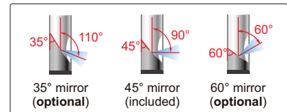
side view (with mirror)
