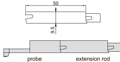
tiny hole probe (optional), code ISR-C002-SBP
