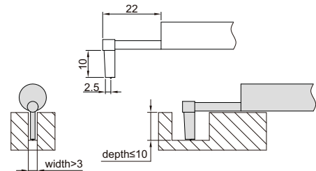
deep groove probe (optional), code ISR-C002-DGP
