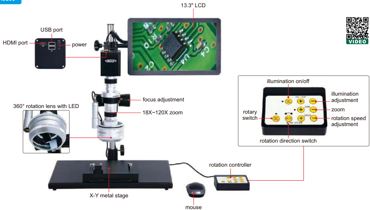
working principle
