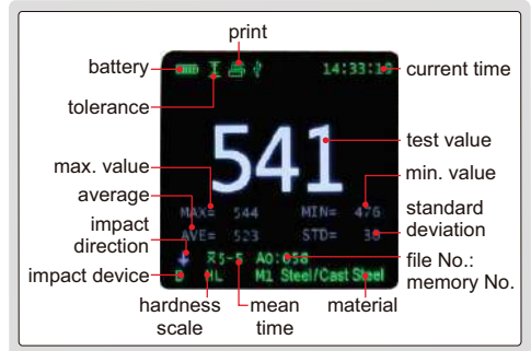
regular display
