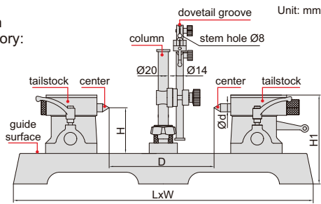
rotary center (optional)
