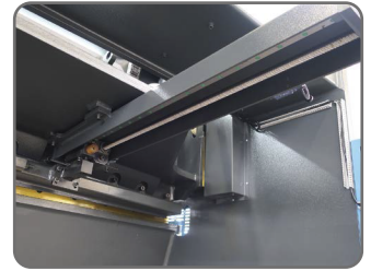
BackGauge with Linear Guide
